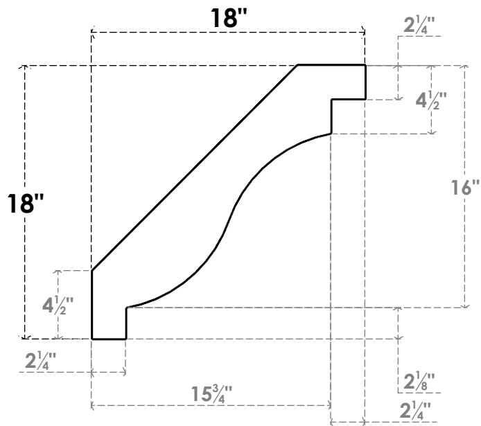
SIDE PROFILE
